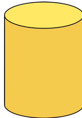
cylinder
