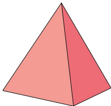
square-based pyramid
