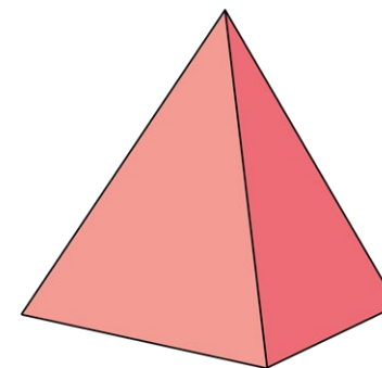
square-based pyramid
