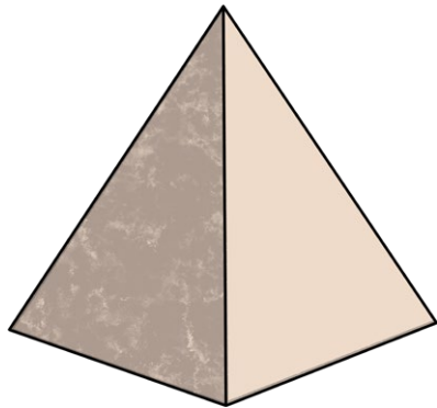
square-based pyramid
