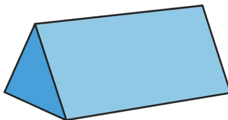
triangular prism
