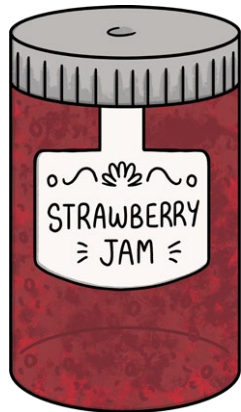
cylinder
