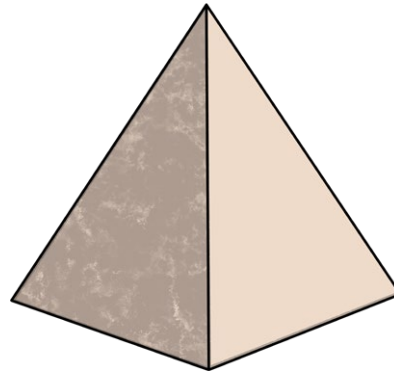
square-based pyramid
