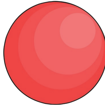
sphere
