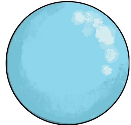
sphere
