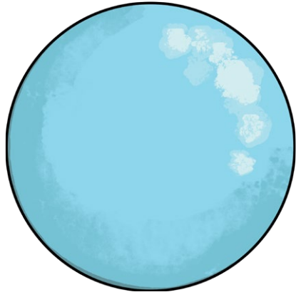
sphere
