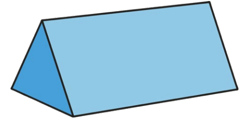
triangular prism
