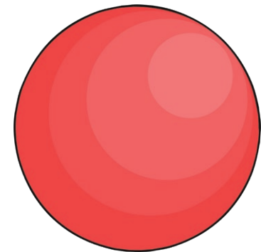
sphere
