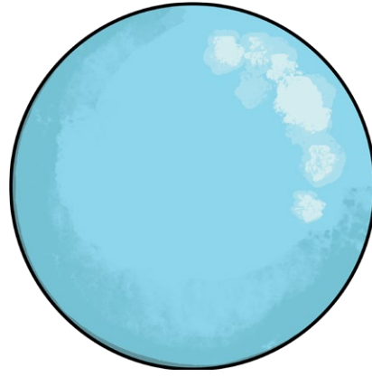
sphere
