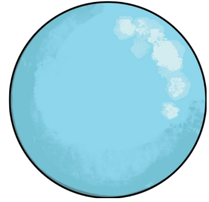
sphere
